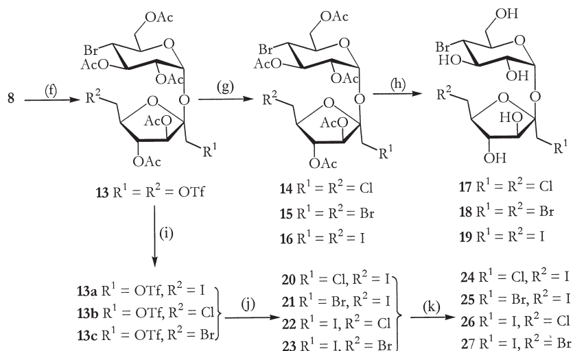
Scheme 2. (f) \text{TiF}_4 , pyridine/ \text{CH}_2\text{Cl}_2 ; (g) 14 : LiCl, acetone, rt, 15 : LiBr, acetone, rt, 16 : KI, acetone, rt; (h) NaOMe, MeOH, rt; (i) 13a : KI, acetone, 0^\circ\text{C} ; 13b : LiCl, acetone, 0^\circ\text{C} ; 13c : LiBr, acetone, rt; (j) 20 : LiCl, acetone, rt, 21 : LiBr, acetone, rt; 22 and 23 : KI, acetone, rt; (k) NaOMe, MeOH, rt.
